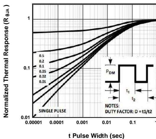
FIG.6-Transient Thermal Impedance
