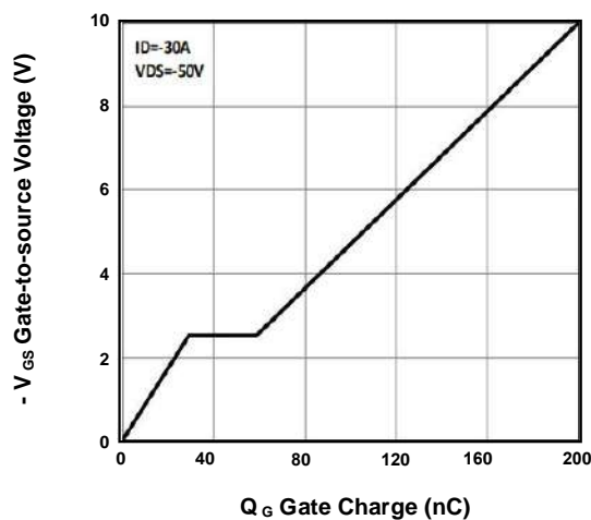
FIG.2-Gate Charge Characteristics
