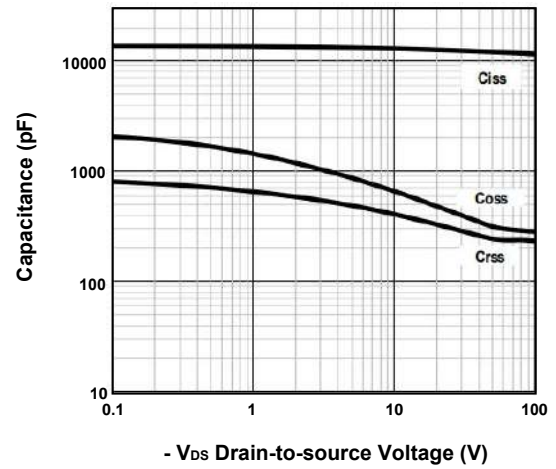
Fig.8-Capacitance Characteristics
