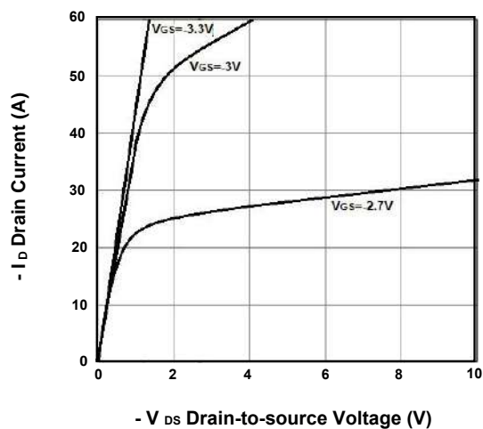
FIG.1-Typical Output Characteristics
