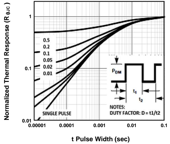
FIG.10-Transient Thermal Impedance
