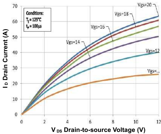
FIG.3- Output Characteristics T_j = 125^\circ\text{C}
