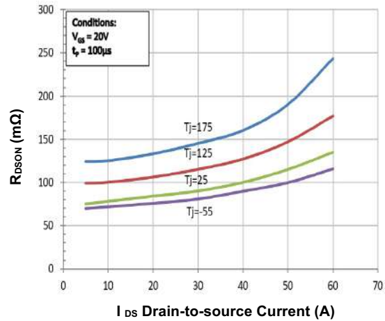
FIG.6- On-Resistance vs. Drain Current For Various Temperature
