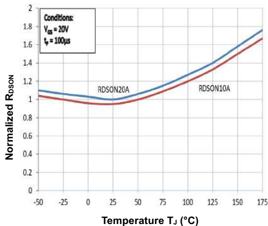
FIG.5-Normalized R_{DS(on)} vs. Temperature T_j
