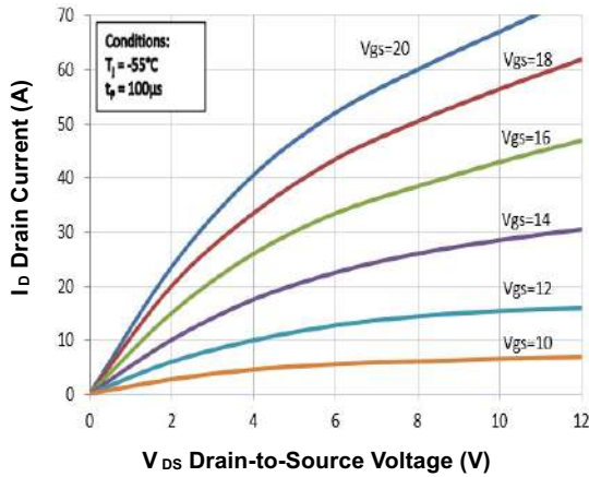
FIG.1-Output Characteristics T_j = -55^\circ\text{C}
