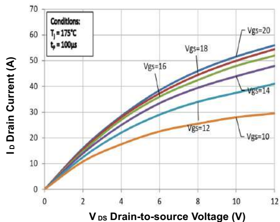
FIG.4- Output Characteristics T_j = 175^\circ\text{C}
